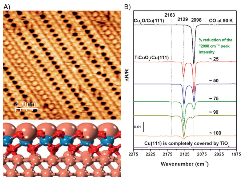
Figure 1. Surface structures of TiCuO x and CO adsorption. A) Atomically resolved STM images of TiCuO x and corresponding DFT simulated surface structures (O red, Ti blue, and Cu reddish-orange). Cu atoms in surface layers are enlarged. B) IRRAS after CO adsorption on TiO x modified surfaces. Peak assignments: 2098 cm -1 CO on Cu 2 O, 2163 cm -1 CO on TiO 2 , 2129 cm -1 CO on TiCuO x .
